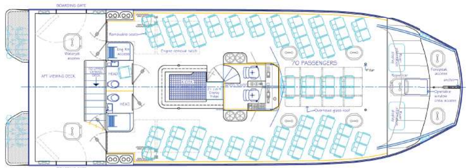
Main Deck Arrangement
